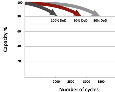
Cyclic life as a function of Depth-Of-Discharge (DoD):
