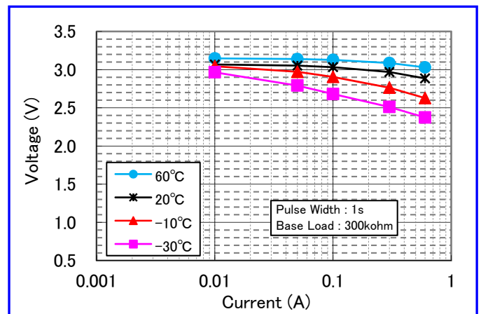
Pulse discharge (D.O.D: 0%)
